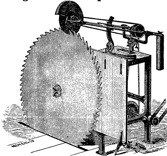
Fig. 2—Rear Prospective View.
